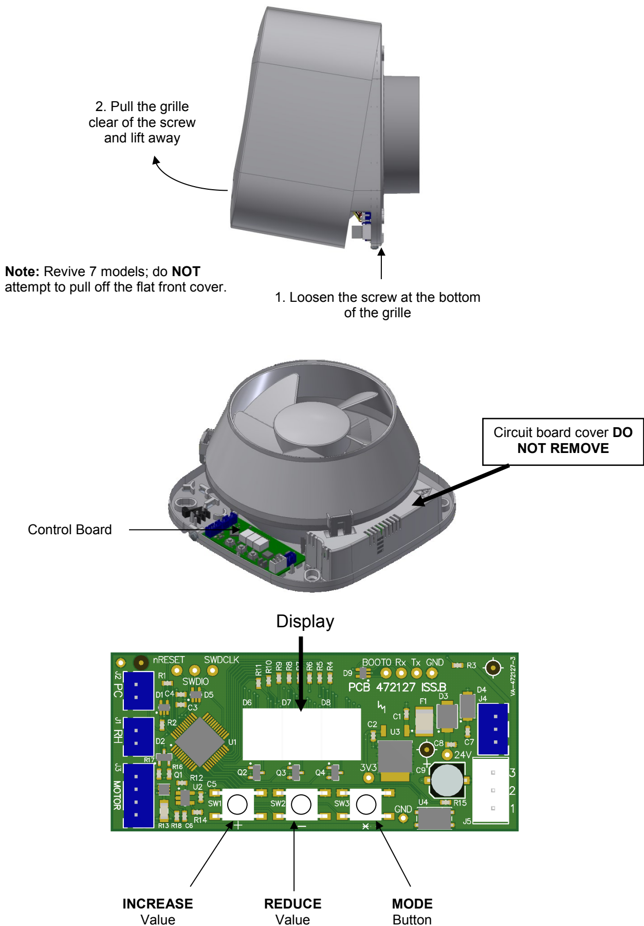
Fig.7. Removing the grille for wiring and setup
